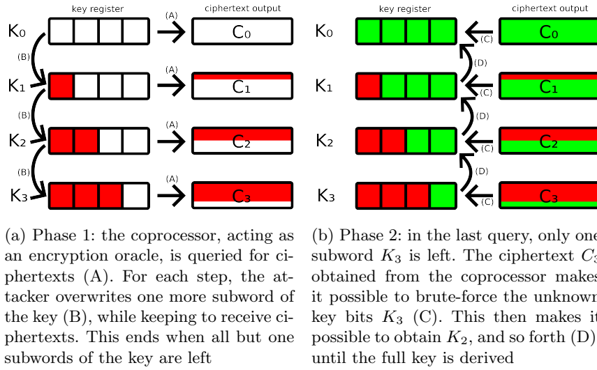
Fig. 1: Diagram of a basic PKO attack on a symmetric-key coprocessor
