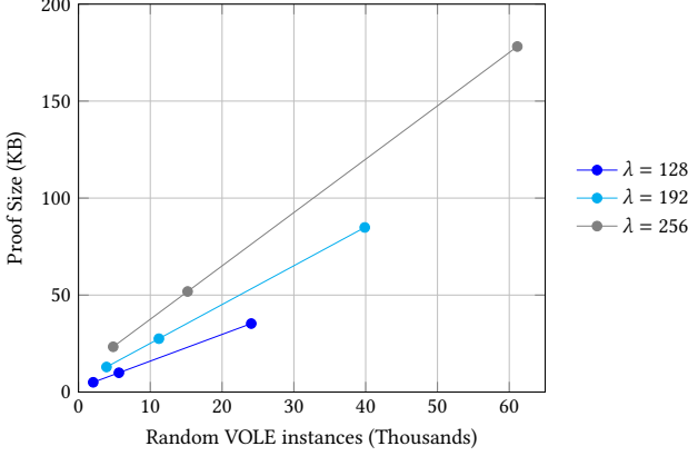
Figure 1: VOLEitH proof size is linearly dependent on the VOLE instances consumed in the proof. Data points for \lambda = 128 are detailed in example 4.1, example 5.10 and example 7.3; these are also shown for higher security levels above.
