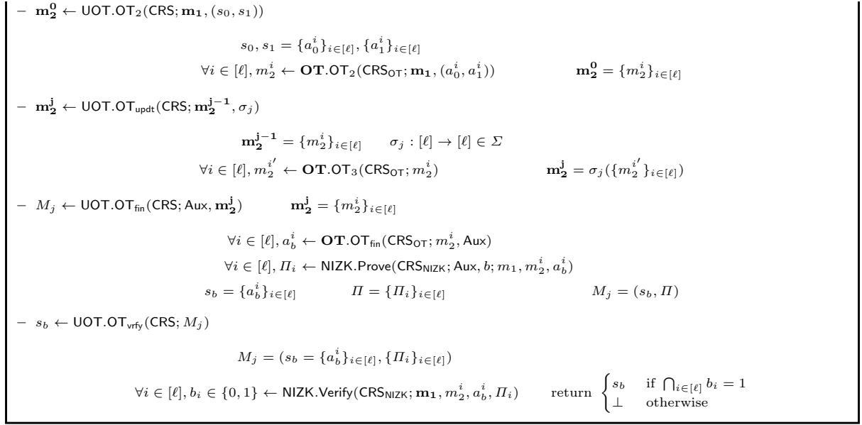
Fig. 13 Construction for \mathcal{F}_{\text{UOT}} using OT
