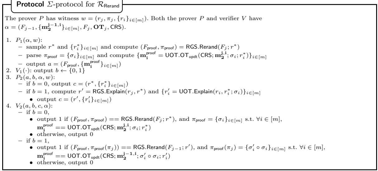
Fig. 15 \Sigma -protocol for Correct Rerandomizing
