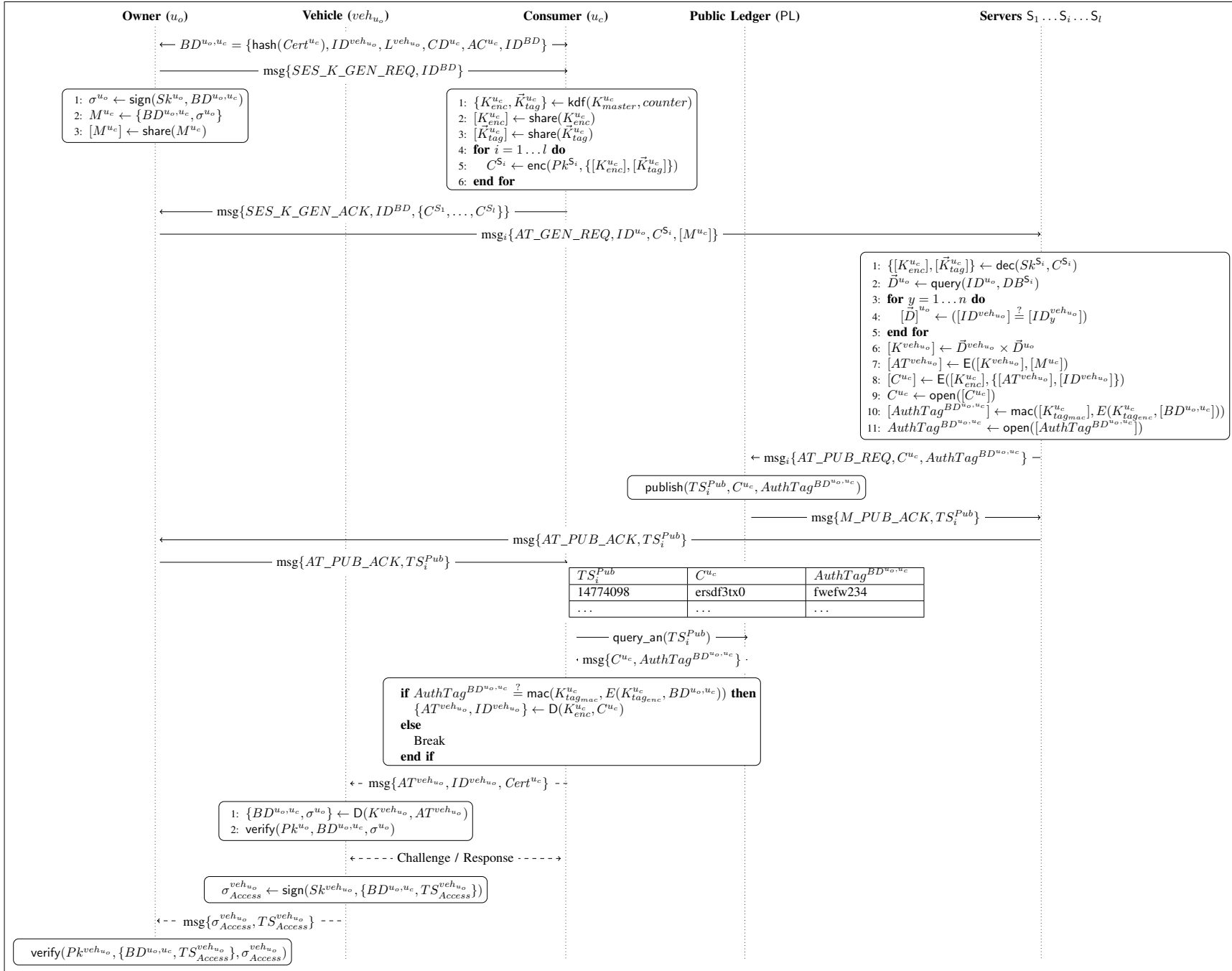
Fig. 9: HERMES complete representation.
