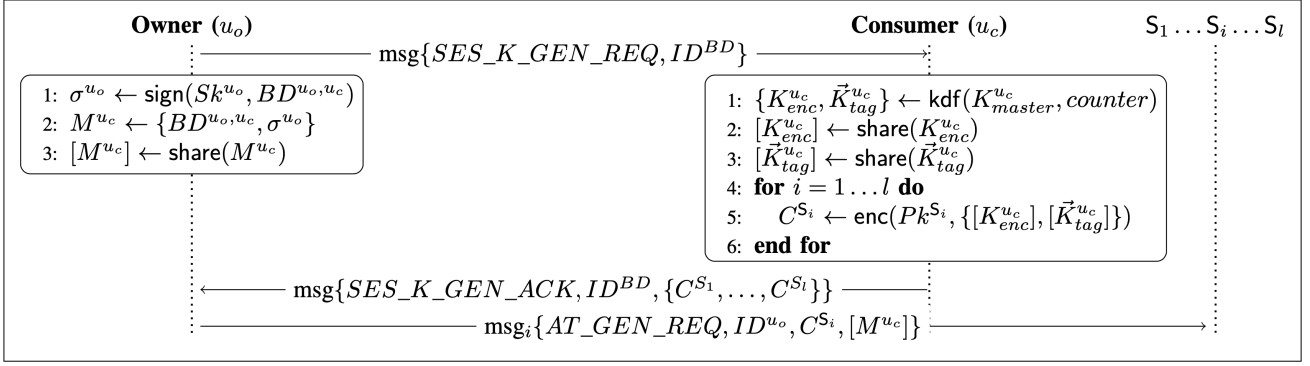
Fig. 3: Step 1: session key generation and BD distribution.
