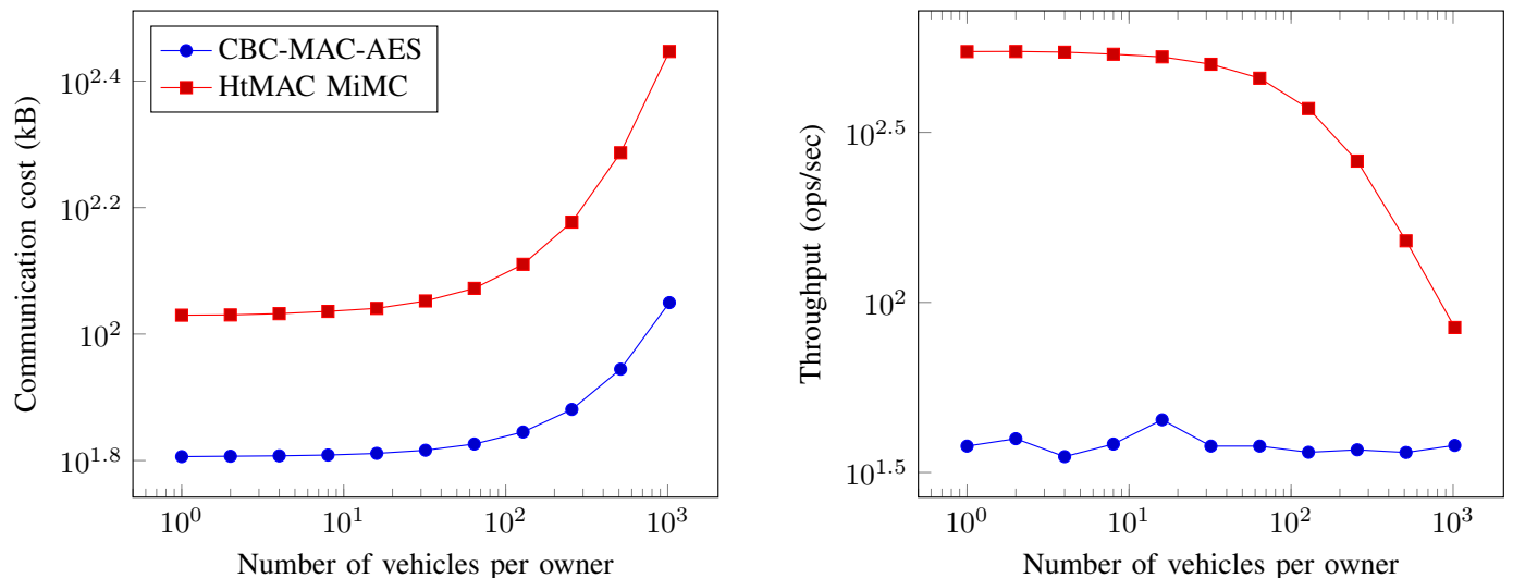
(a) Communication cost per server: The intra-VSSP communication cost for Access Tokens (ATs) generation (i.e., data sent-received). (b) Throughput for all servers: The throughput of all servers in VSSP for Access Tokens (ATs) generation (i.e., ops) per second.
