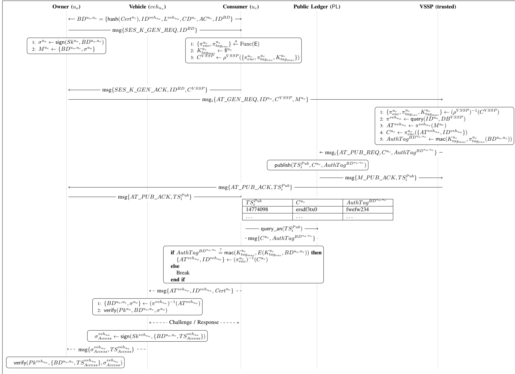
Fig. 10: Simplified representation of HERMES for the proof of Theorem 2.
