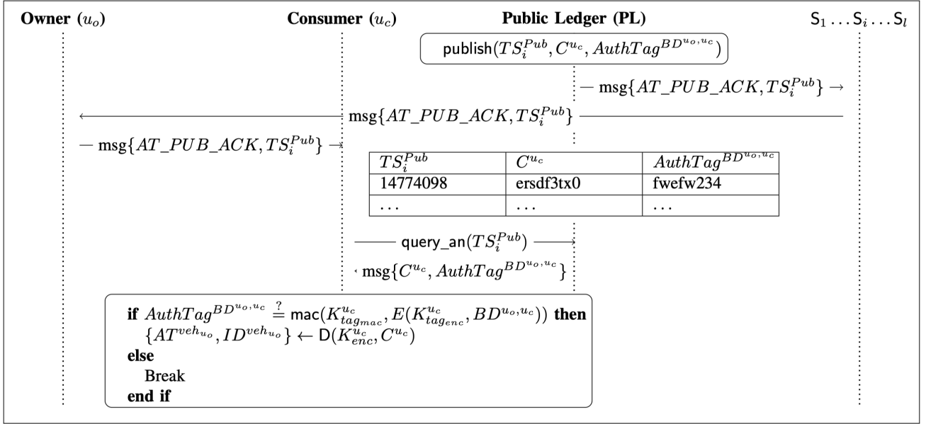
Fig. 5: Step 3: Access token distribution and verification.
