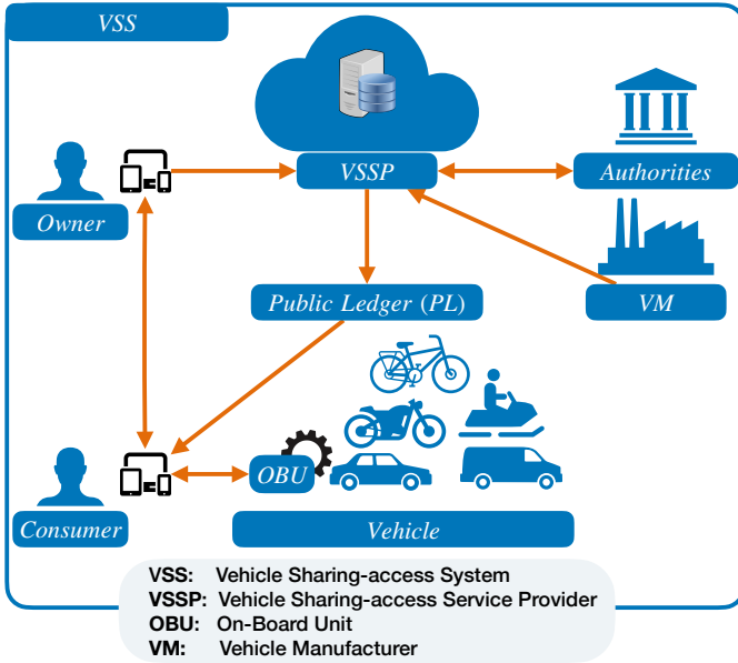
Fig. 1: Vehicle Sharing-access System (VSS) model.
