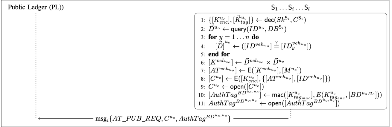
Fig. 4: Step 2: AT generation.
