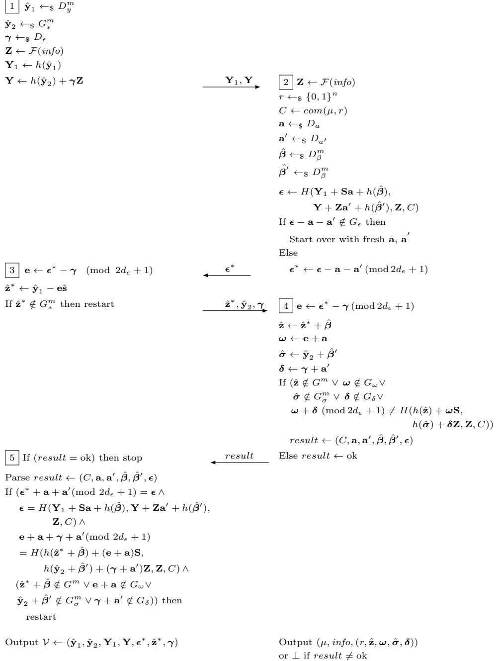
Fig. 1. The five-step, four-move signature issuing protocol (steps shown in boxed numbers) for the proposed PBSS. All parameter and set definitions are given in Table 1. For brevity, we omit any verifications performed by the two parties w.r.t. the domains from which the protocol messages come from.
