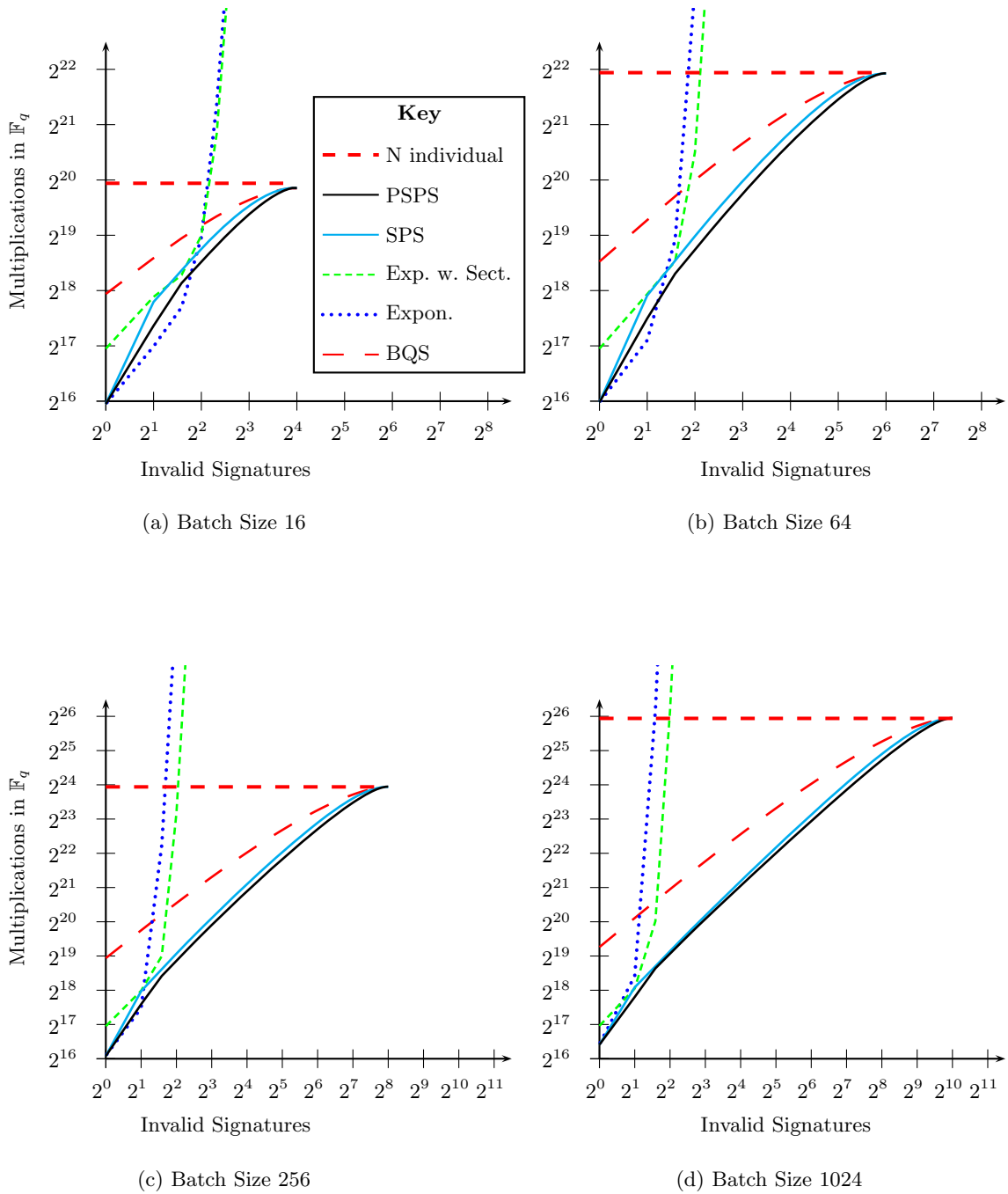
Fig. 2: Number of multiplies in F_q , where r and q are 256-bit values and d = 12 .
