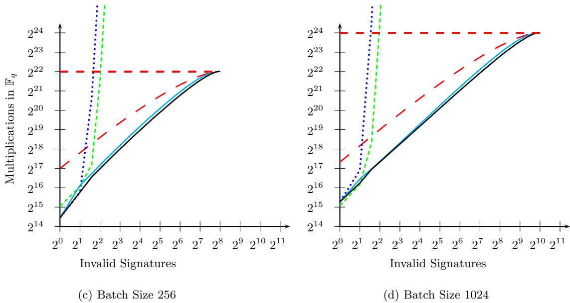
Fig. 1: Number of multiplies in F_q , where r and q are 160-bit values and d = 6 .
