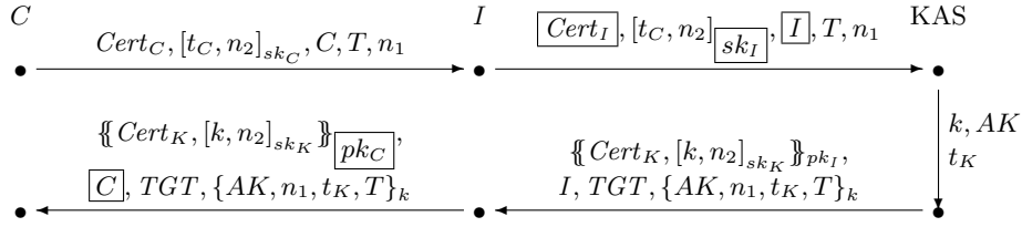
Fig. 2. Message Flow in the Man-In-The-Middle Attack on PKINIT-26
