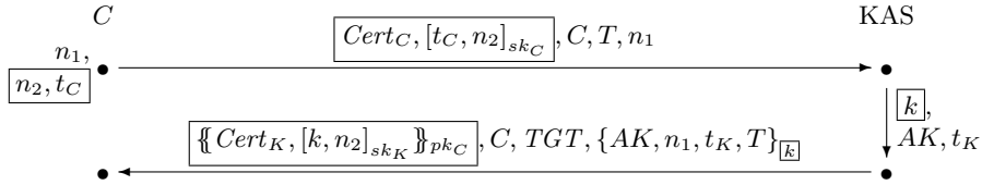
Fig. 1. Message Flow in the Traditional AS Exchange and in PKINIT-26
