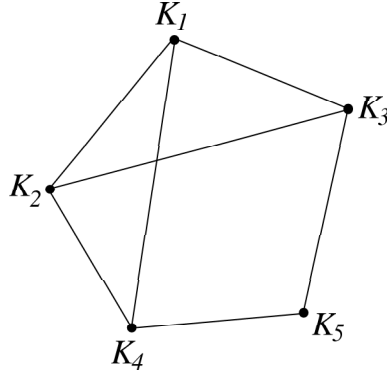
Figure 2: The \mathcal{S}' -secants for Case B
