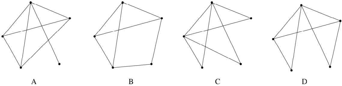
Figure 1: The 4 cases for the \mathcal{S}' -secants
