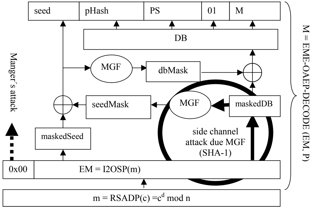
Fig. 1: New side channel attack against RSA-OAEP
